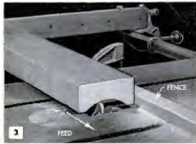
It is practical to use a saw blade for cove cuts up to about 45 deg., as above. The cuts are about 1/8 in. deep per pass. Below, the molding head is a true cutter and will cut any angle up to 90 deg. With it, cuts can be as deep as 1/2 in. per pass. The molding head performs better, but the saw can be very useful
